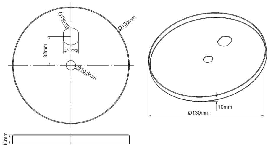
Ceiling Canopy
