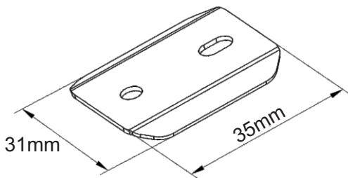
LAP-Connector
